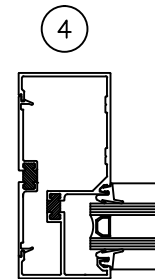
PART# TWJ450 WALL JAMB PART# T-FF200 FLAT FILLER
