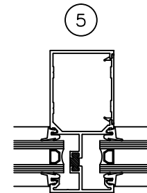
PART# TOV452 VERTICAL PART# OHF450 POCKET FILLER
