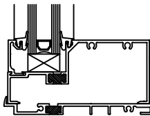
PART# TSM450/ST SILL W/STOP PART# TSF-200 SILL FLASHING
