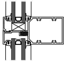
PART# TOH450/ST TUBULAR HORIZONTAL
