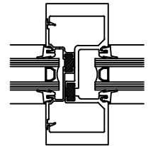
PART# TH452 HEAVY VERTICAL PART# TEIF200 POCKET FILLER
