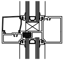
PART# TEH450/ST TUBULAR HORIZONTAL
