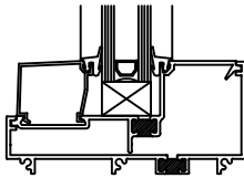
PART# TSC450 SILL CAN PART# TSI450/ST SILL INSERT W/STOP
