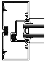
PART# TEV452 JAMB W/SPLINE PART# T-FF200 FLAT FILLER
