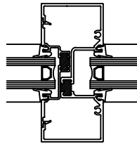
PART# TEV452 VERT W/SPLINE PART# TEIF200 POCKET FILLER
