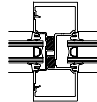
PART# TIV452 INTERMEDIATE VERTICAL PART# TEIF200 POCKET FILLER
