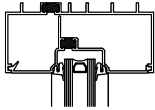
PART # THC450 HEAD CAN PART # THI450 HEAD INSERT
