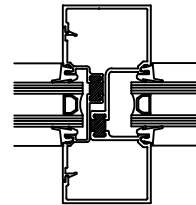
PART# TEV452R VERT NO SPLINE PART# TEIF200 POCKET FILLER
