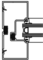
PART# TEV452R JAMB NO SPLINE PART# T-FF200 FLAT FILLER
