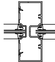
PART# V152 VERT W/SPLINE PART# F100 POCKET FILLER
