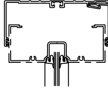
OPTIONAL TWO PIECE HEAD CAN
