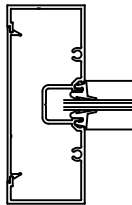
PART# V152 JAMB W/SPLINE PART# FF200 FLAT FILLER
