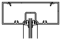
PART # V152 HEAD W/SPLINE PART # FF200 FLAT FILLER
