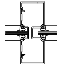
PART# V157 VERT NO SPLINE PART# F100 POCKET FILLER
