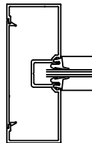
PART# V157 JAMB NO SPLINE PART# FF200 FLAT FILLER
