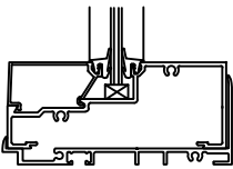
PART# H153/ST SILL W/STOP PART# SF200 SILL FLASHING
