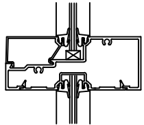
PART# H153/ST OPEN HORIZ W/STOP PART# F100 POCKET FILLER
